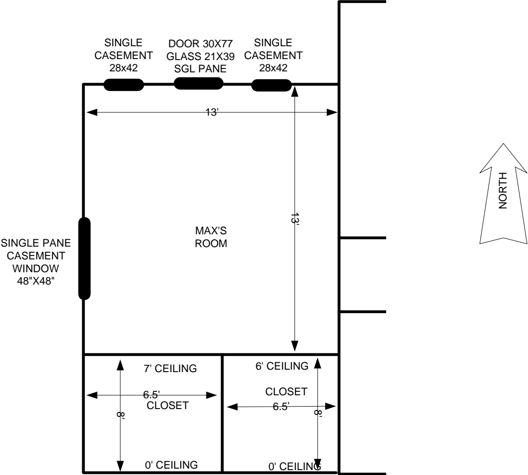
2nd FLOOR-WEST
